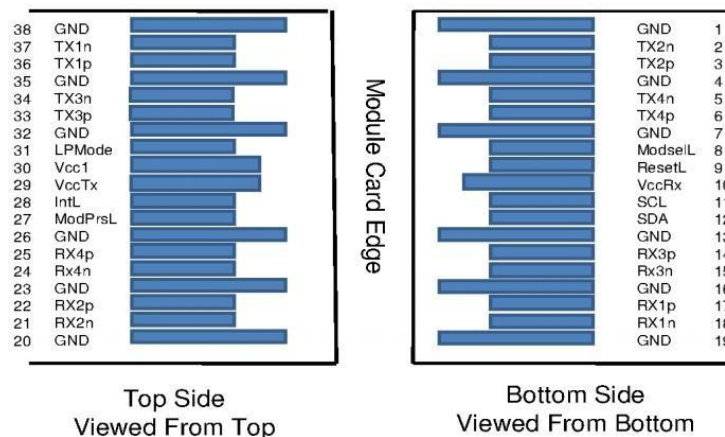
Figure1 Top Side and Bottom Side of QSFP28
