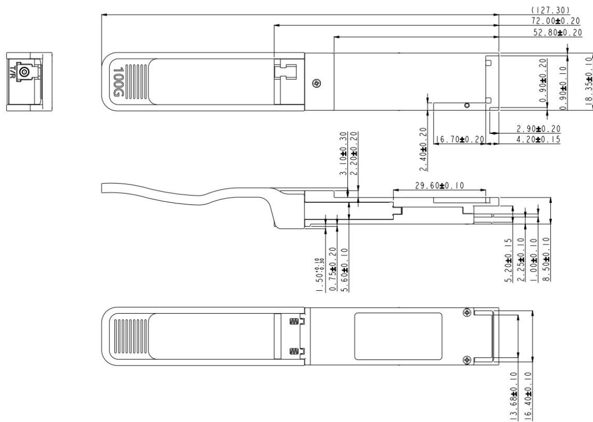
Figure3 100G LR1 BIDI QSFP28 Mechanical Dimensions
